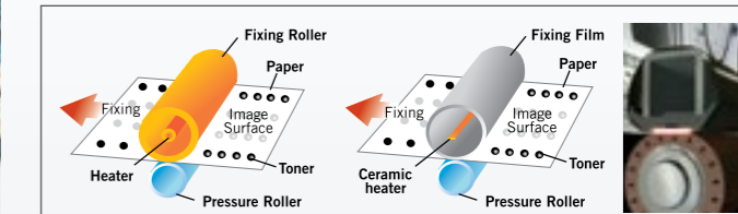
Conventional Roller Fixing Method
